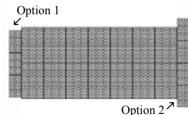
Fig. 10 Plan view showing the end rows turned perpendicular. The corners may not match up perfectly, so two acceptable alternatives are shown. Most plans do not show this configuration. Field adjustments are easily made.
