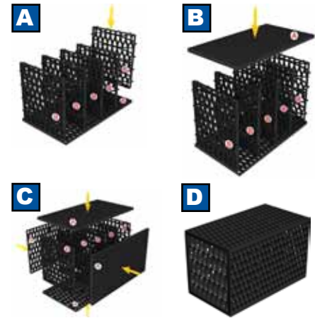
Figure 2 Follow these steps to assemble a 5-plate R-Tank HD .
