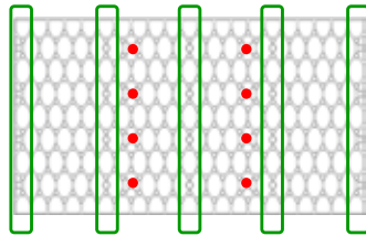
Fig. 1 For standard R-Tank HD units attach small plates at locations circled in green, do not use the holes indicated in red.
